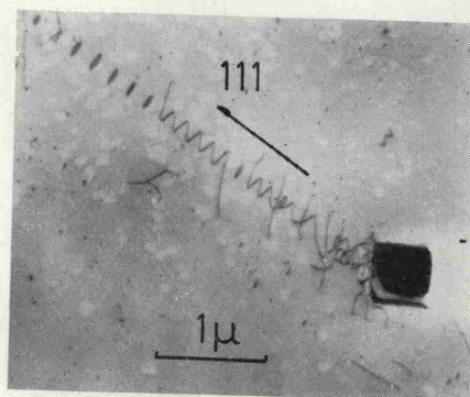
A classical prismatic dislocation source, observed by transmission electron microscopy, in polycrystalline chromium after pressurization at 15 kbars.
